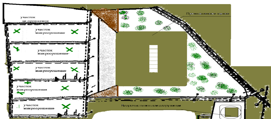
Fig.1. Scheme of the irrigation sprinkling station on the experimental part of the Tertersky RWCN in the Garabagh land in the period 2006-2010 with the use of the Idad and MDR sprinklers:
