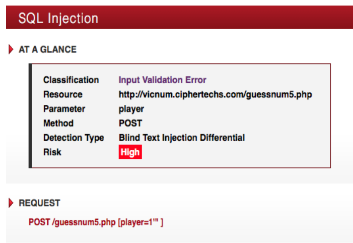
Figure 7: VEGA scan of 1 SQL Injection from Vicnum
