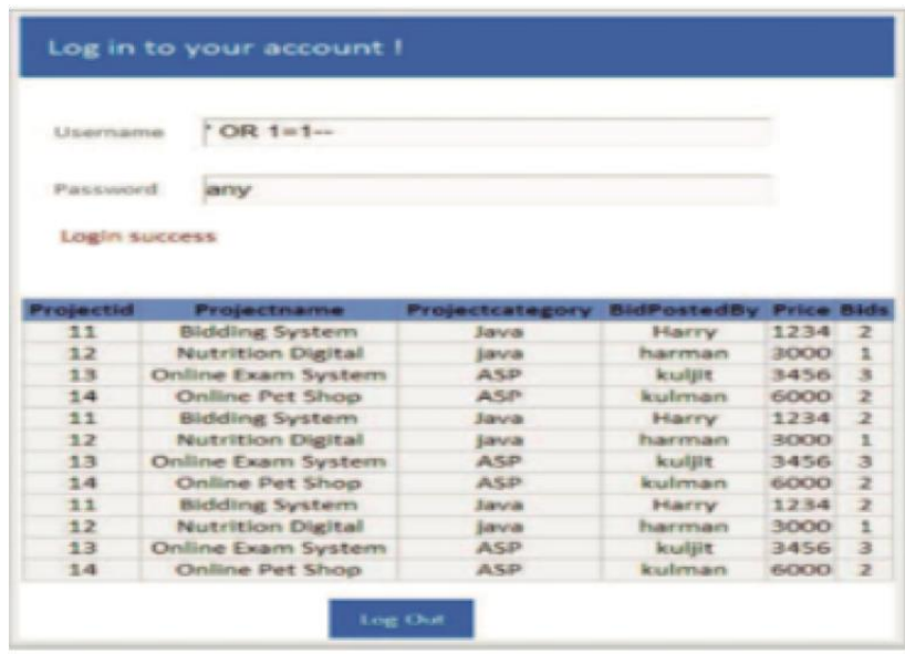
Figure 1: SQL Injection where a hacker logs in and retrieves all the sensitive data
